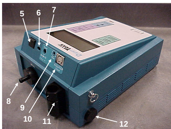
Figure 1–1: Top and Front of the DUSTTRAK Monitor
